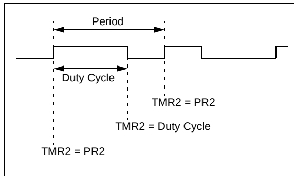
FIGURE 11-4: PWM OUTPUT
